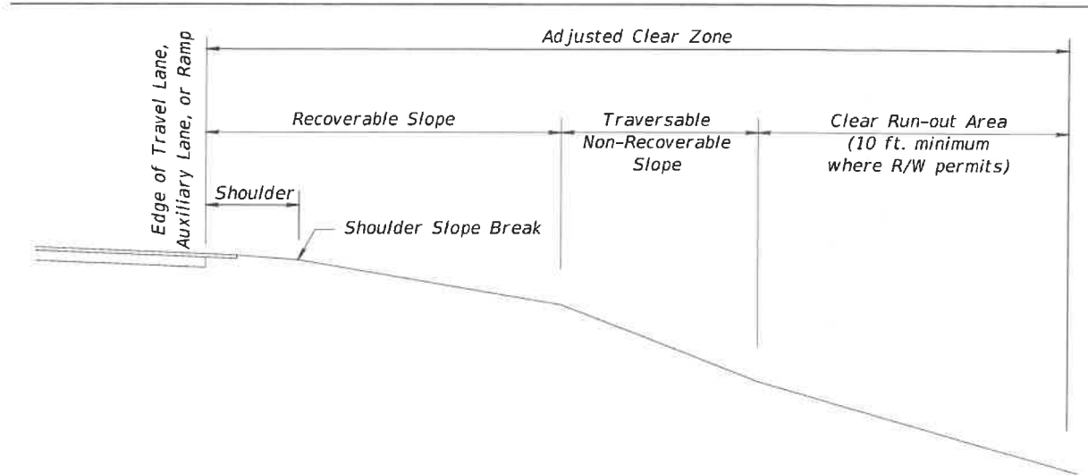
Figure 215.2.3 Adjusted Clear Zone Concept
