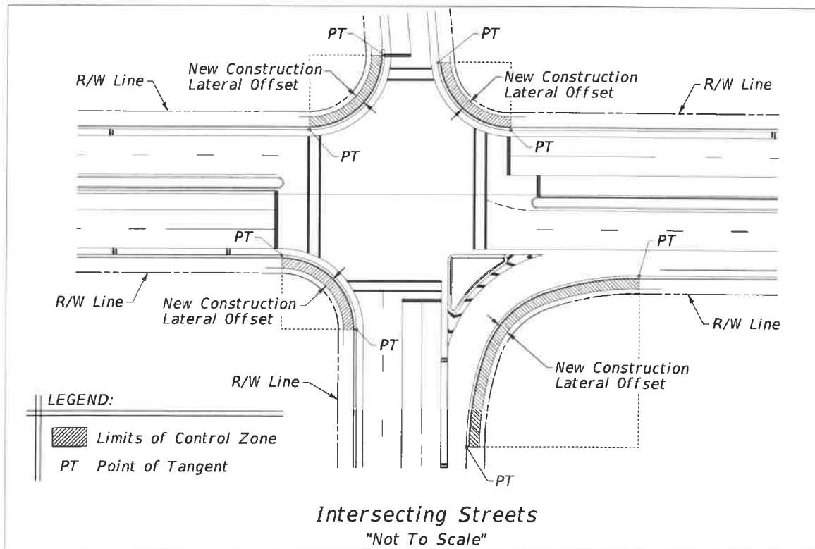
Figure 215.2.4 Intersection Radii
