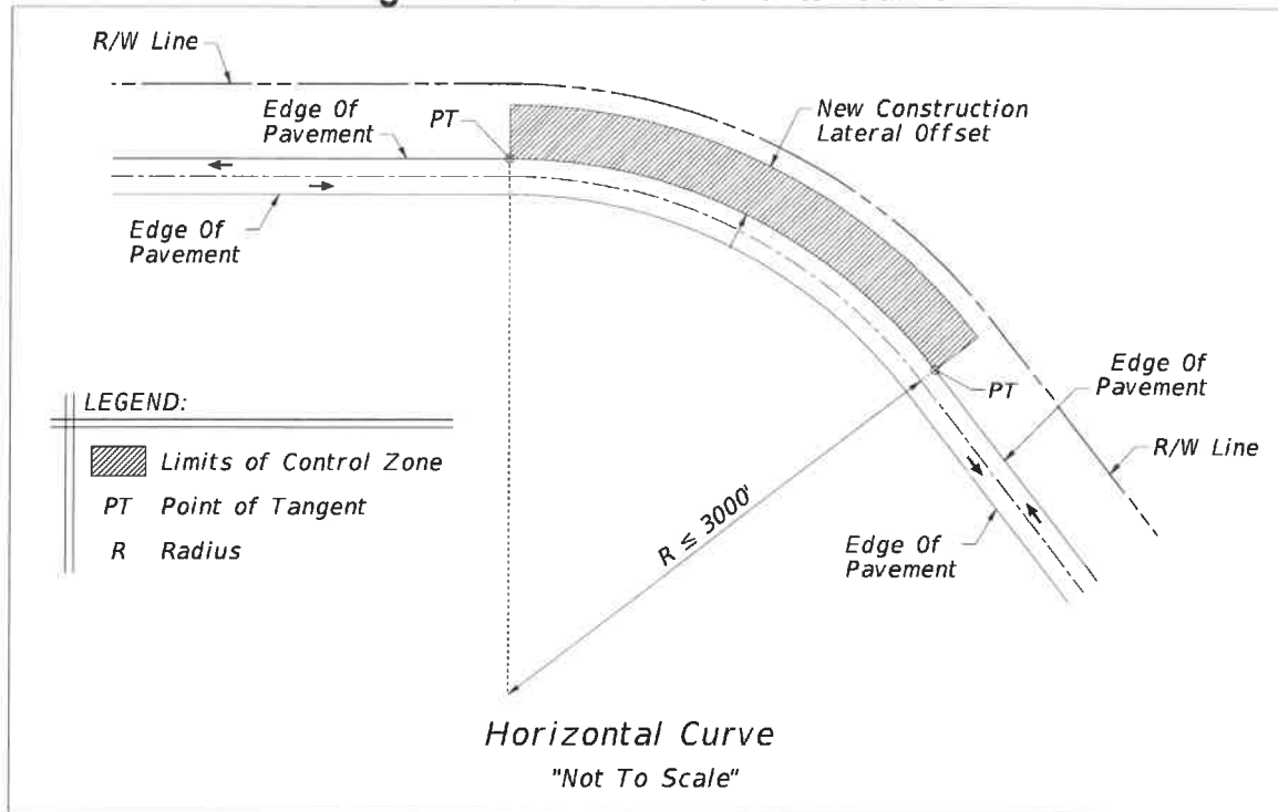
Figure 215.2.12 Horizontal Curve
