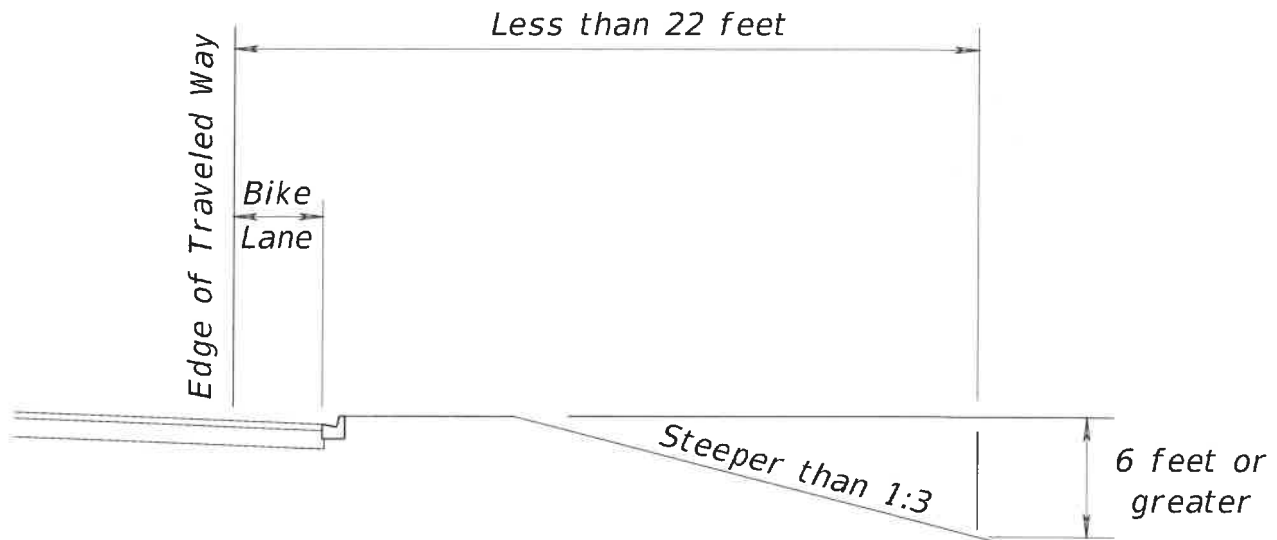
Figure 215.3.3 Drop-off Hazard on Curbed Roadways
